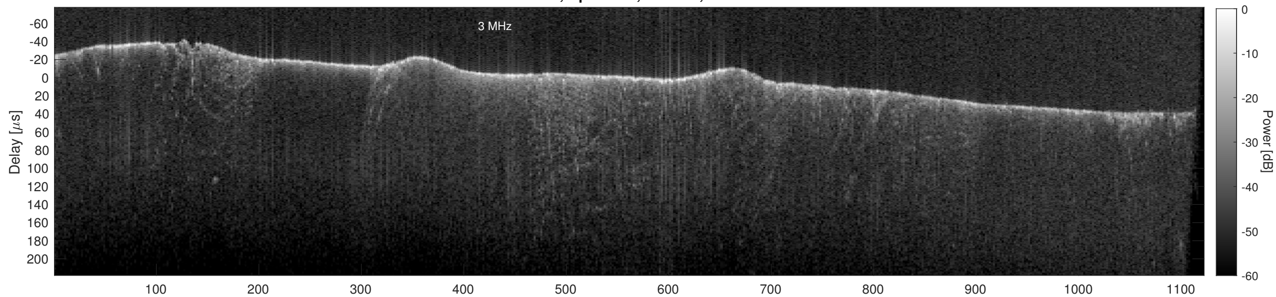
Orbit 12216, Cluttergram
