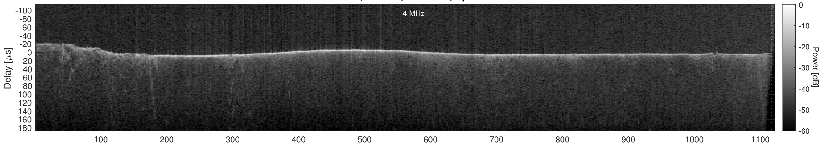
Orbit 12217, Cluttergram
