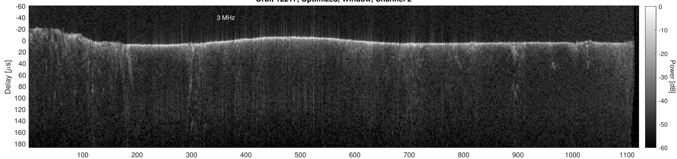
Orbit 12217, Cluttergram
