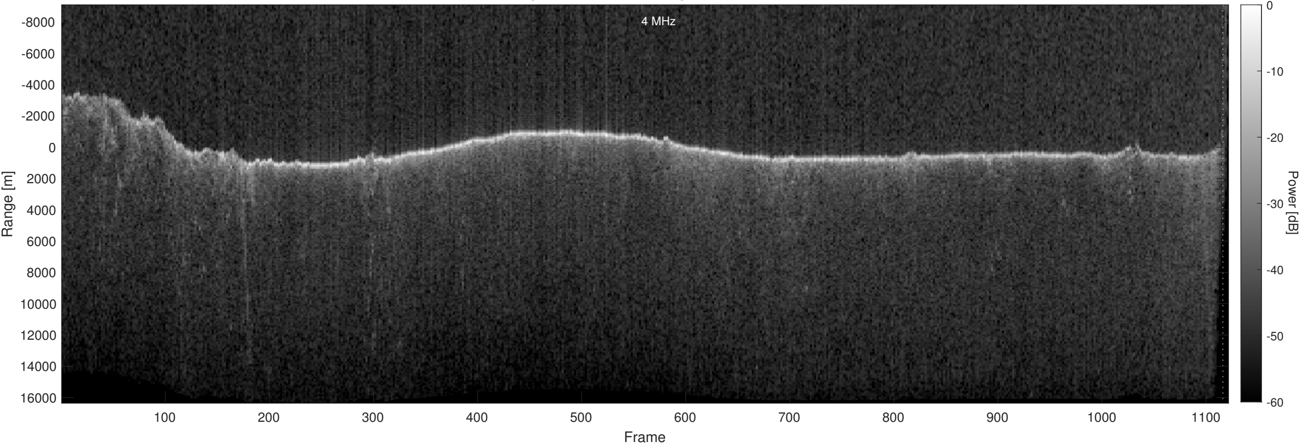
Orbit 12217, Optimized, Window, Depth-Corrected, Channel 2
