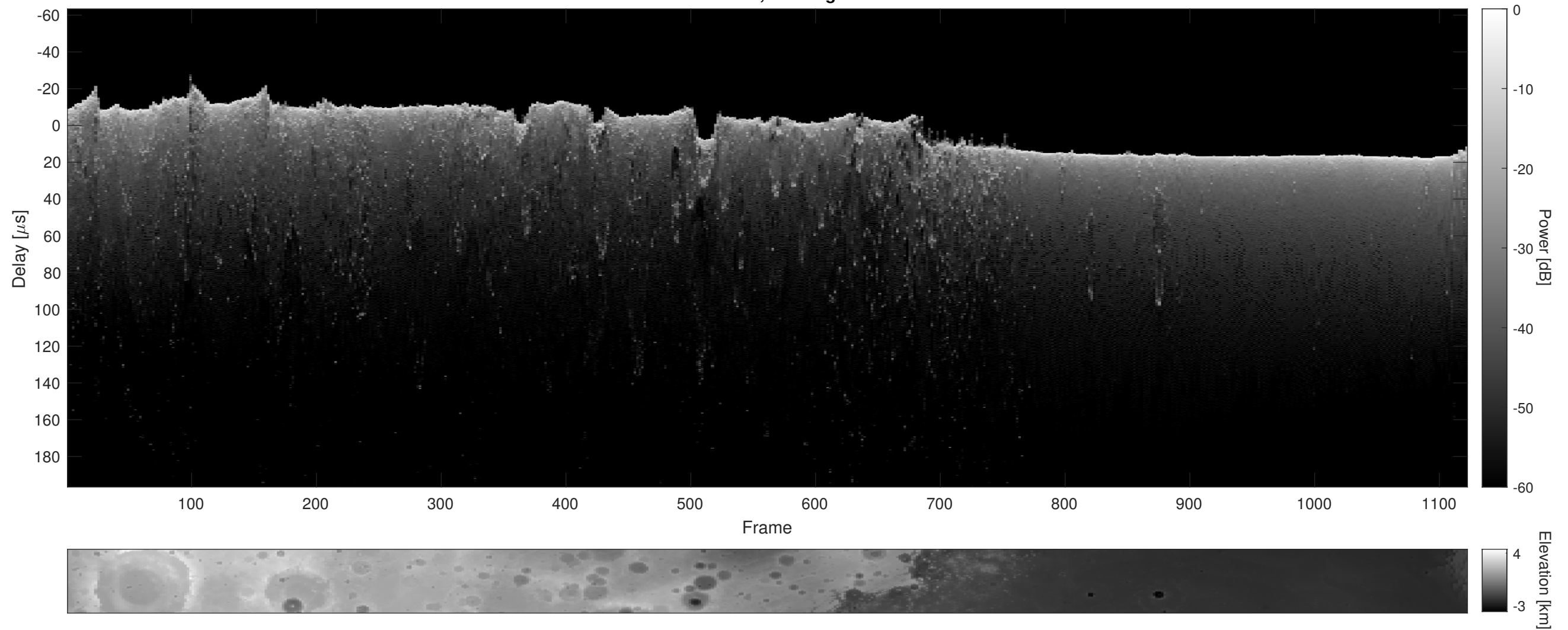
Orbit 12218, Cluttergram
