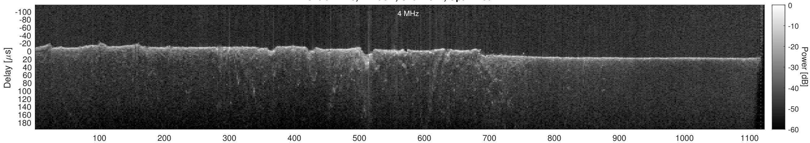
Orbit 12218, Cluttergram
