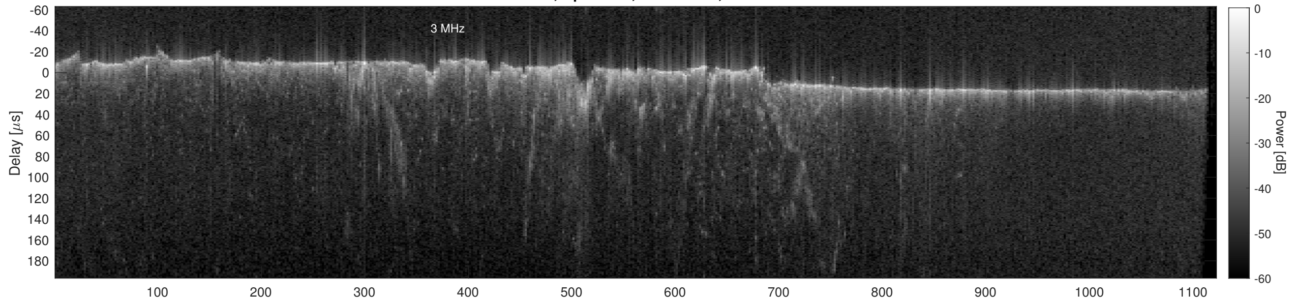
Orbit 12218, Cluttergram
