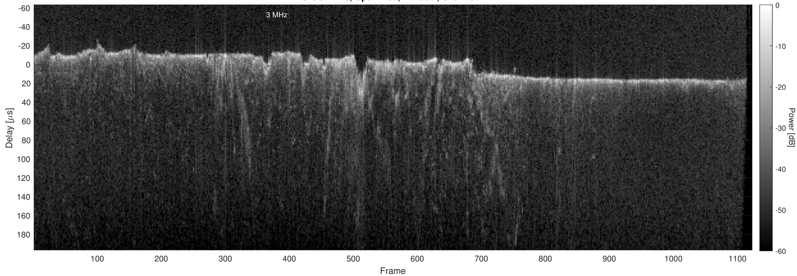
Orbit 12218, Optimized, Window, Channel 2
