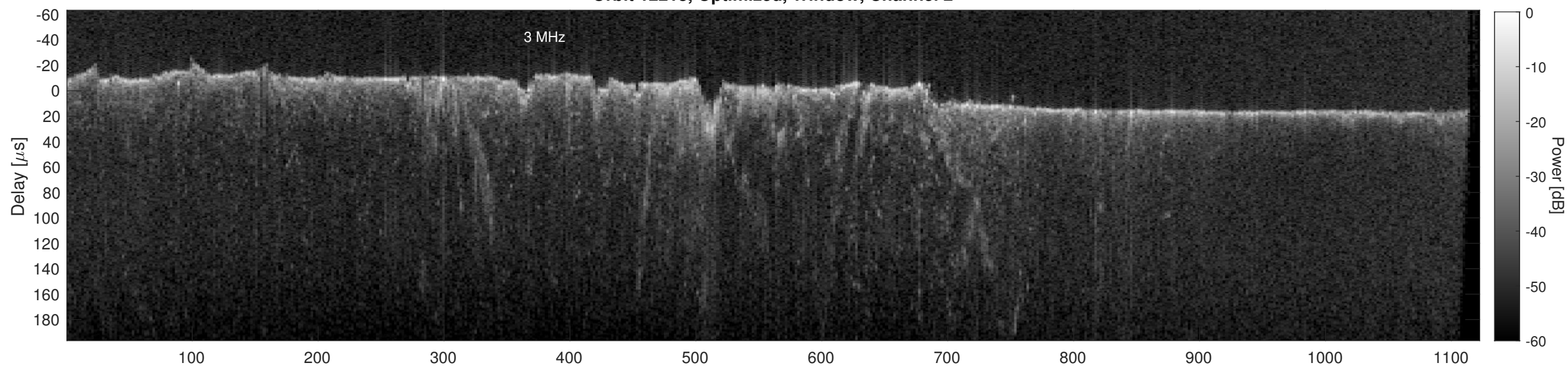
Orbit 12218, Cluttergram
