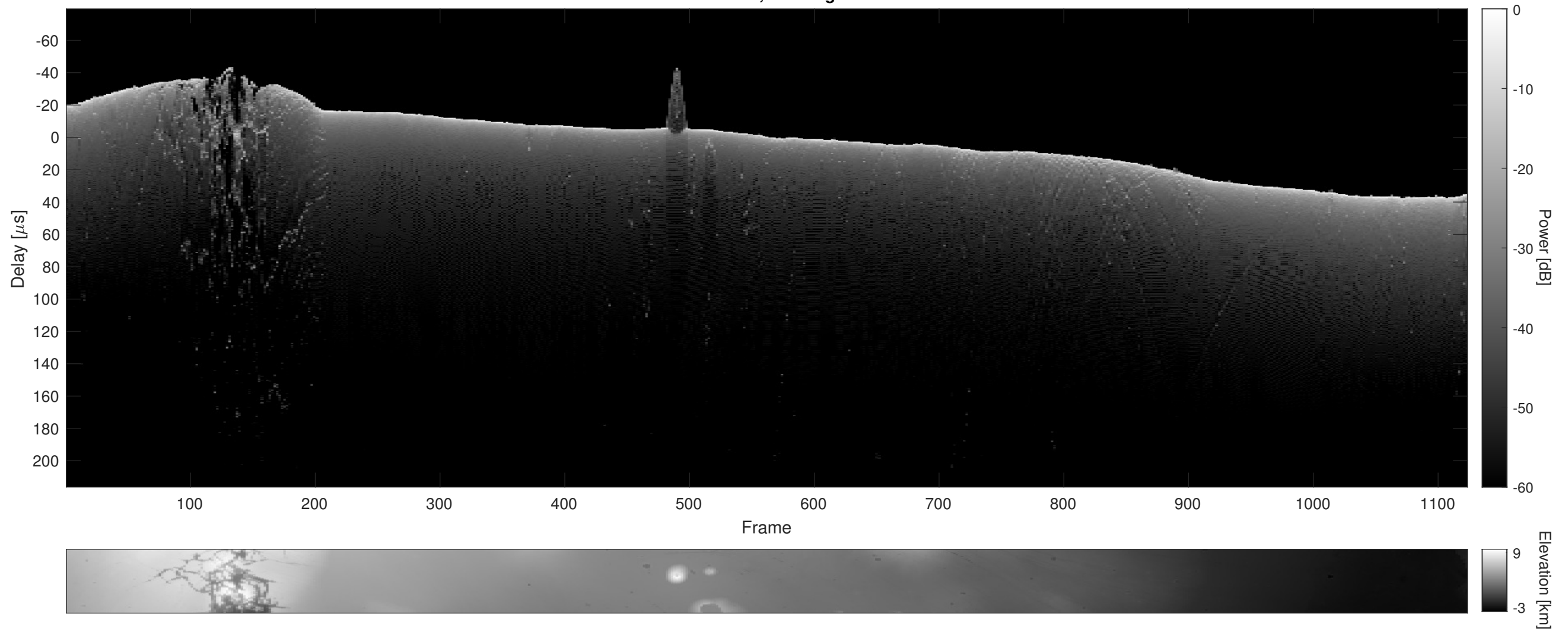
Orbit 12223, Cluttergram
