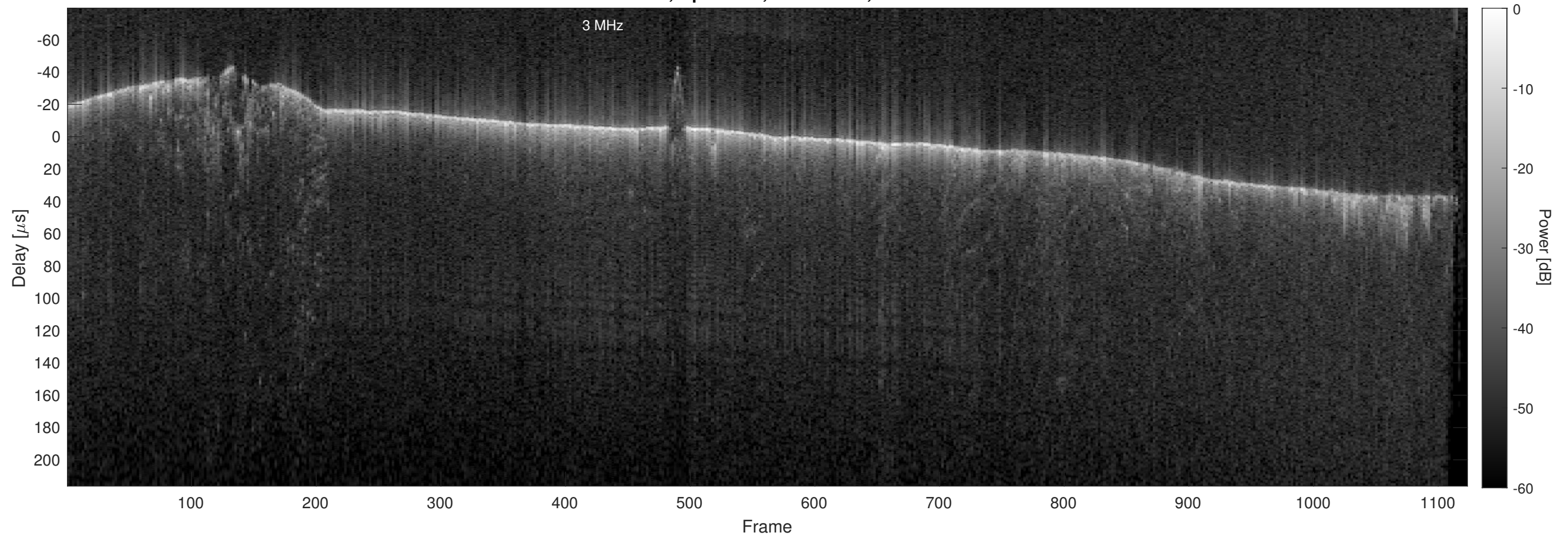
Orbit 12223, Optimized, No Window, Channel 2
