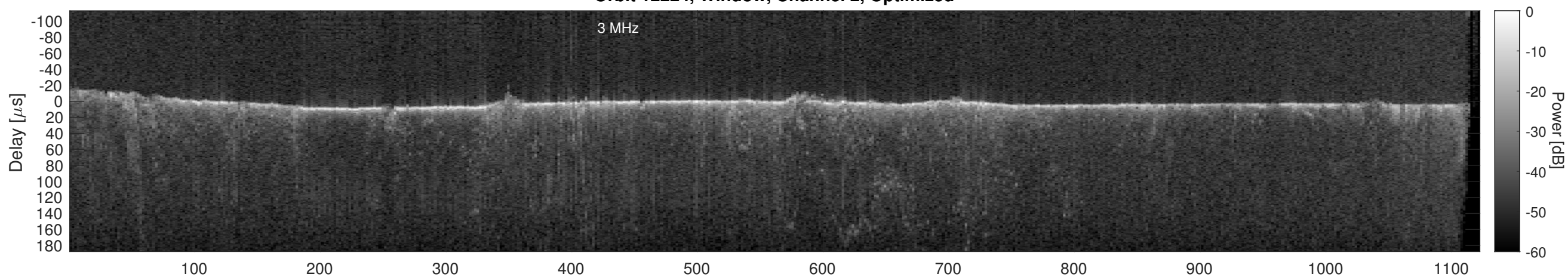
Orbit 12224, Cluttergram
