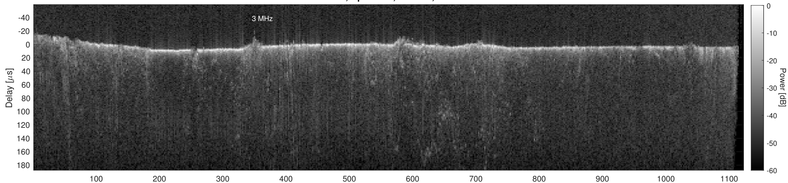
Orbit 12224, Cluttergram
