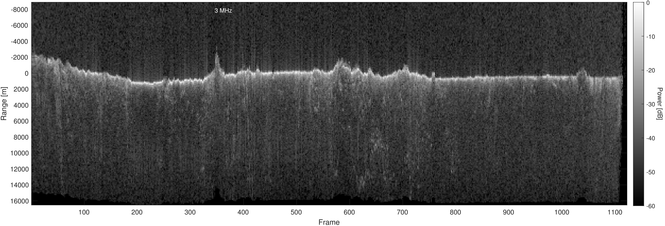
Orbit 12224, Optimized, Window, Depth-Corrected, Channel 2
