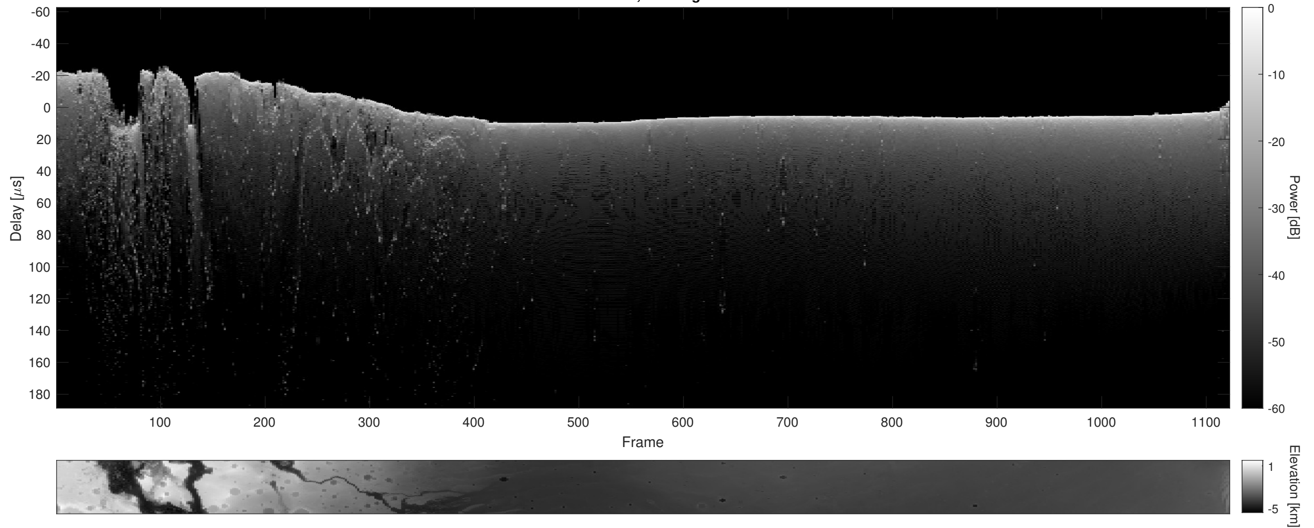
Orbit 12226, Cluttergram
