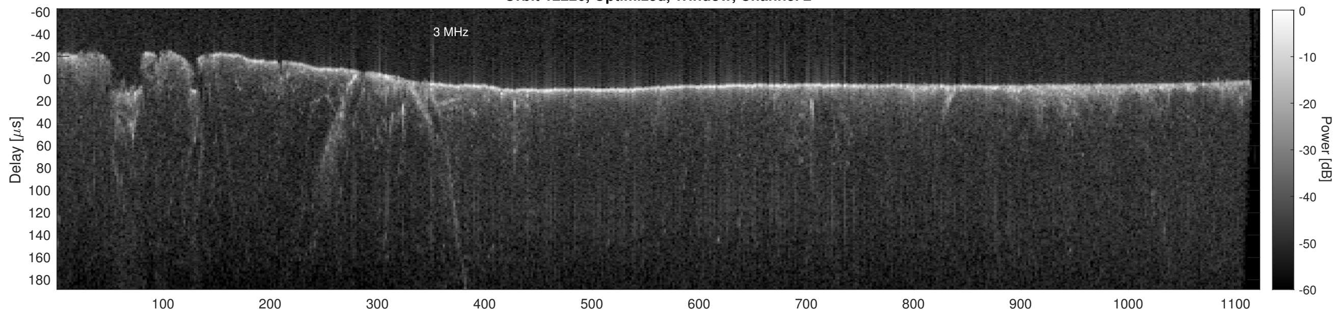
Orbit 12226, Cluttergram
