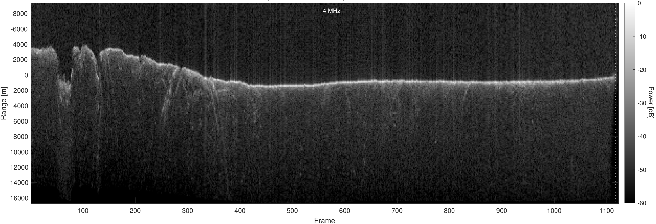
Orbit 12226, Optimized, Window, Depth-Corrected, Channel 2
