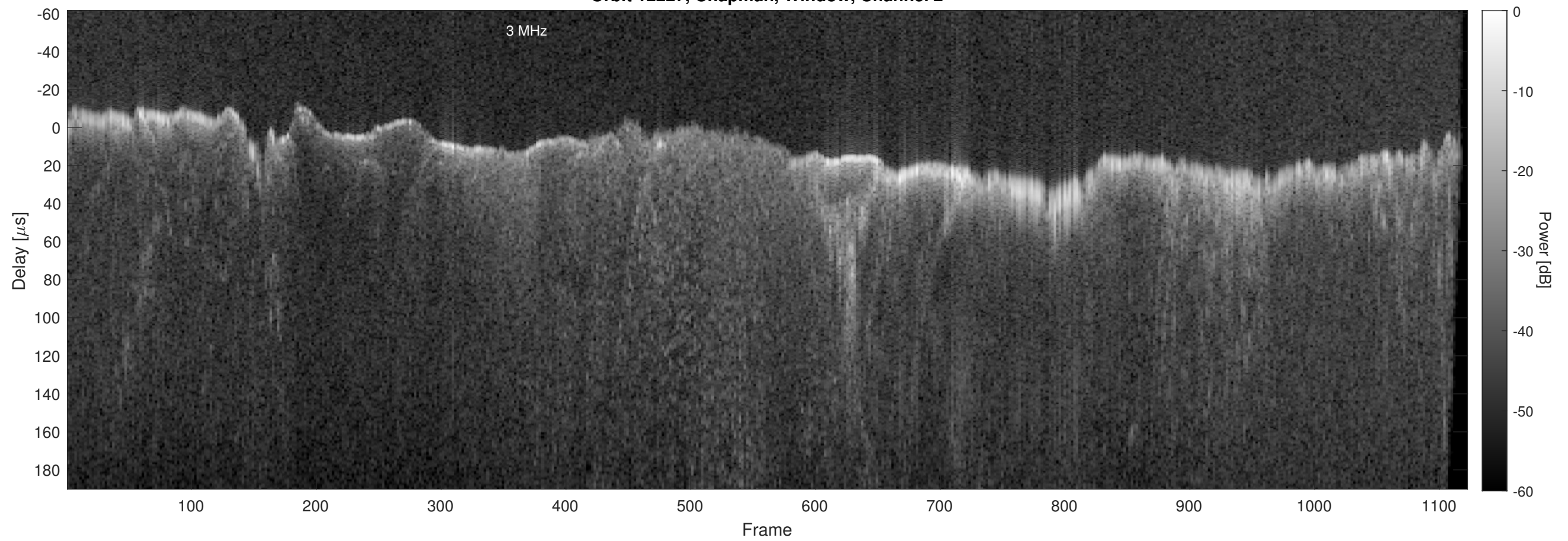
Orbit 12227, Chapman, Window, Channel 2
