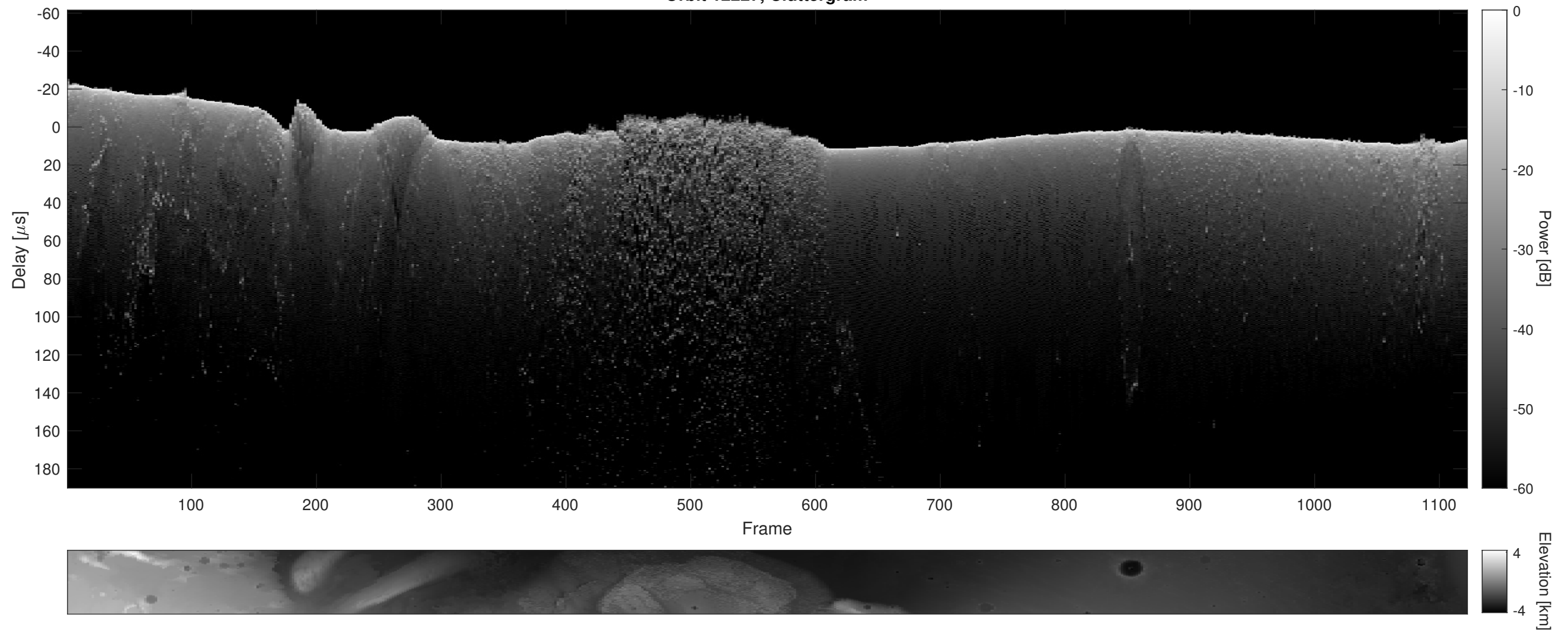
Orbit 12227, Cluttergram
