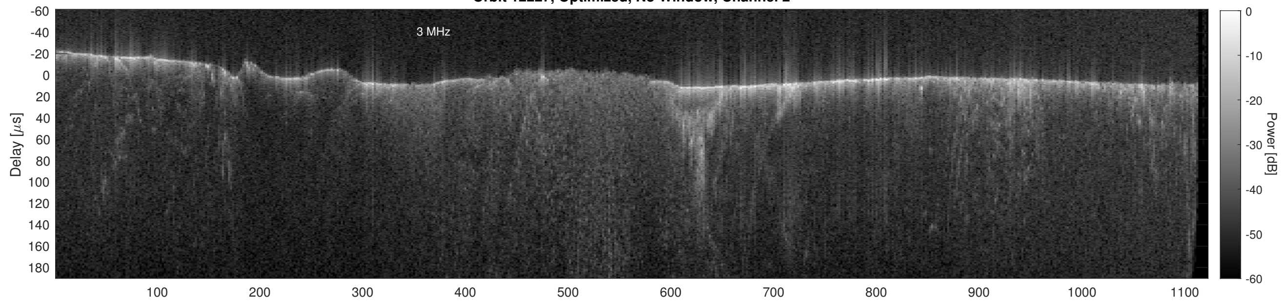
Orbit 12227, Cluttergram
