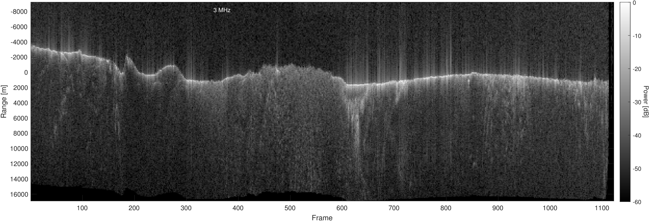
Orbit 12227, Optimized, No Window, Depth-Corrected, Channel 2
