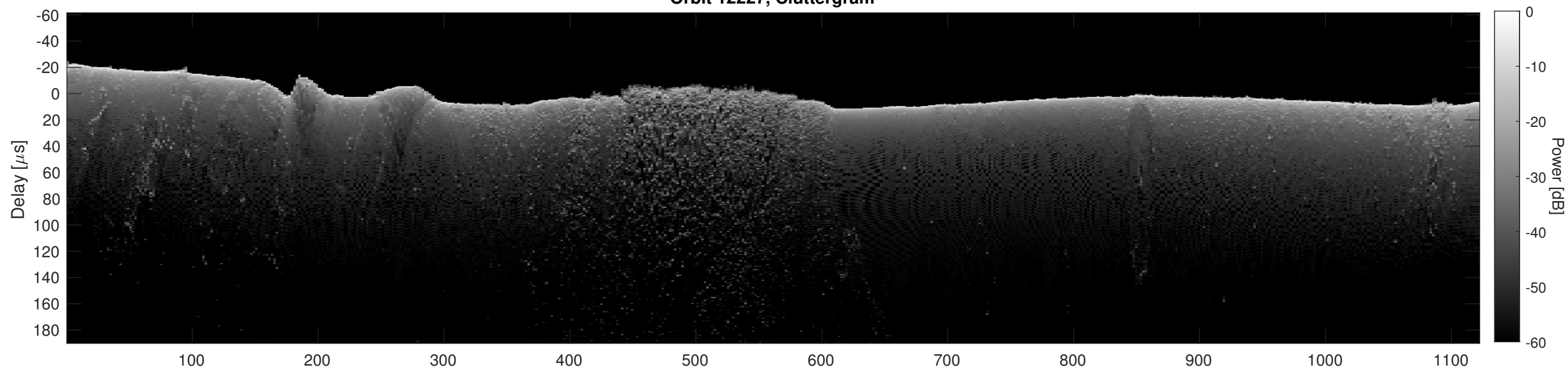
Orbit 12227, Cluttergram
