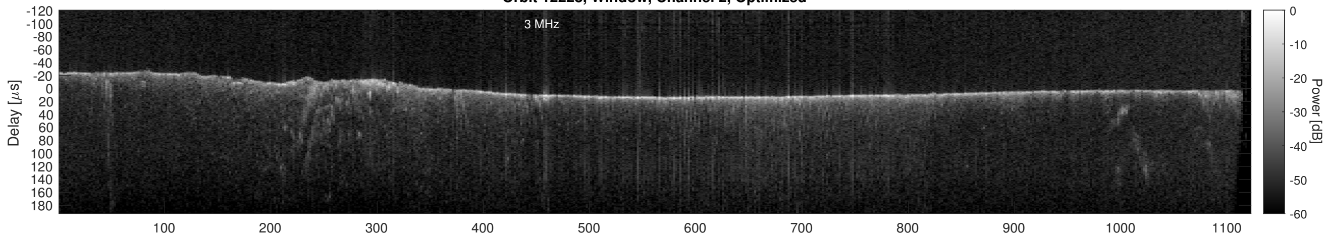
Orbit 12228, Cluttergram
