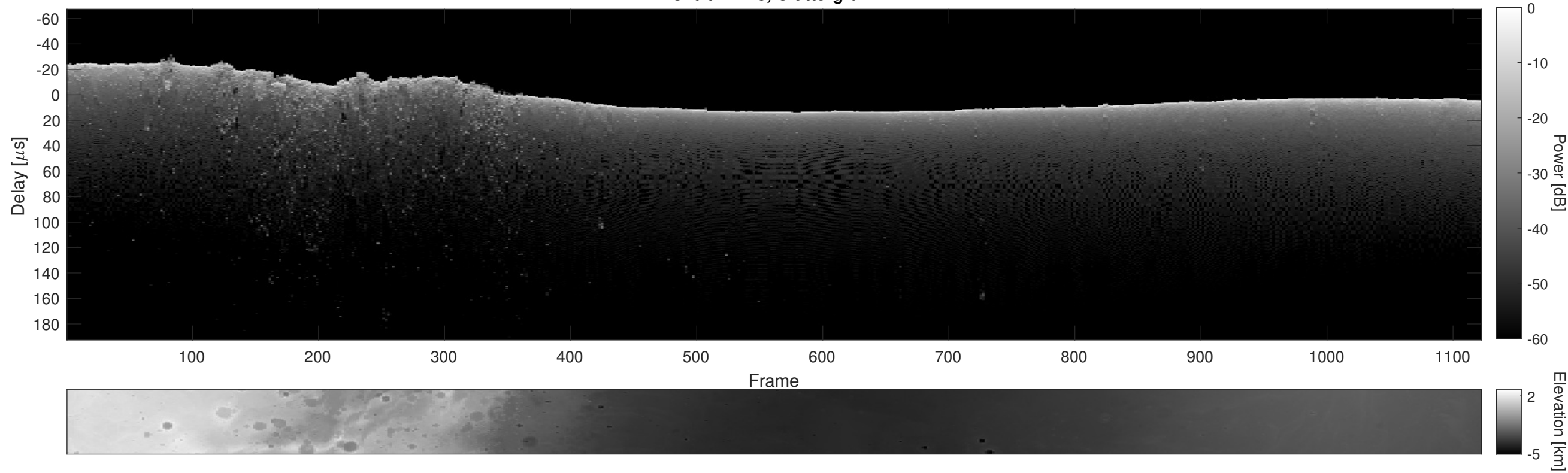
Orbit 12228, Cluttergram
