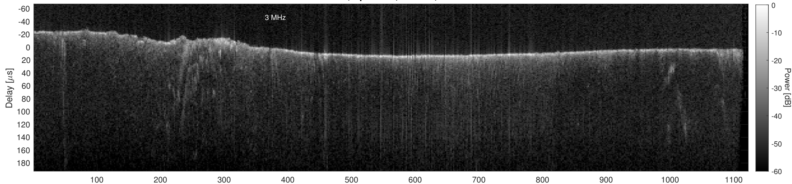
Orbit 12228, Cluttergram
