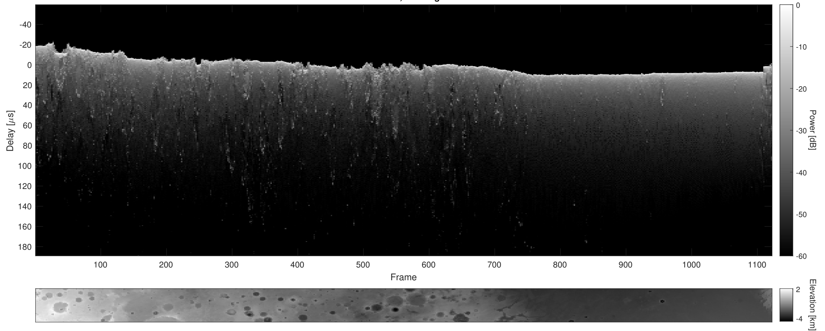
Orbit 12229, Cluttergram
