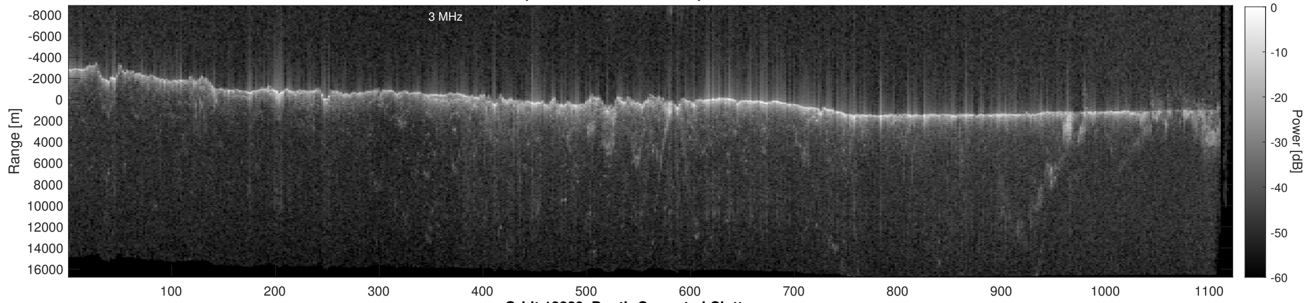
Orbit 12229, Depth-Corrected Cluttergram
