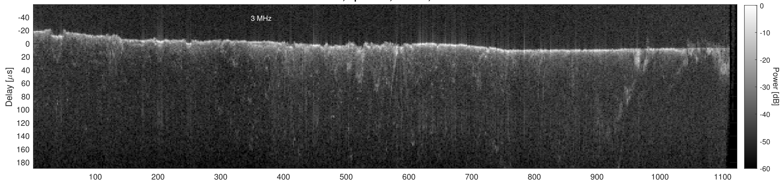
Orbit 12229, Cluttergram
