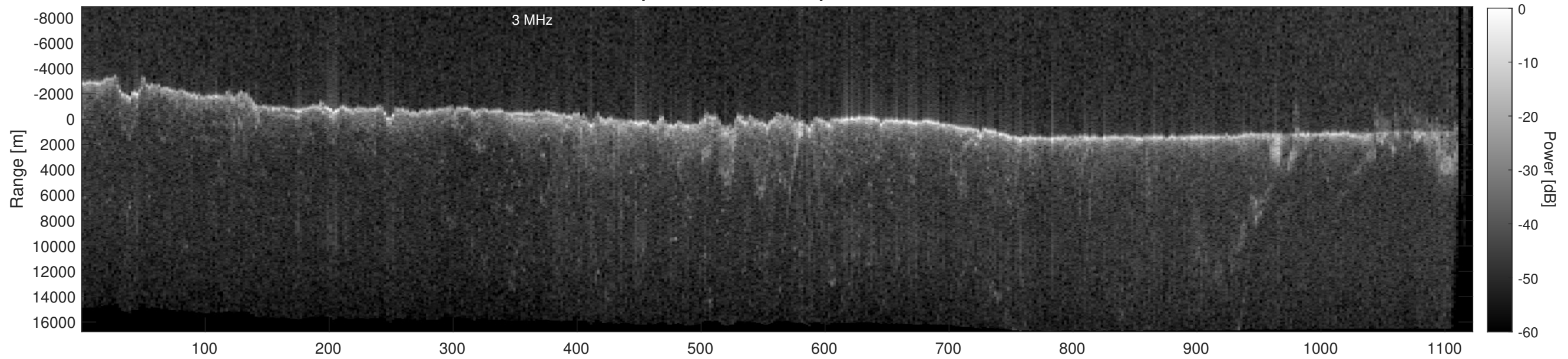
Orbit 12229, Depth-Corrected Cluttergram
