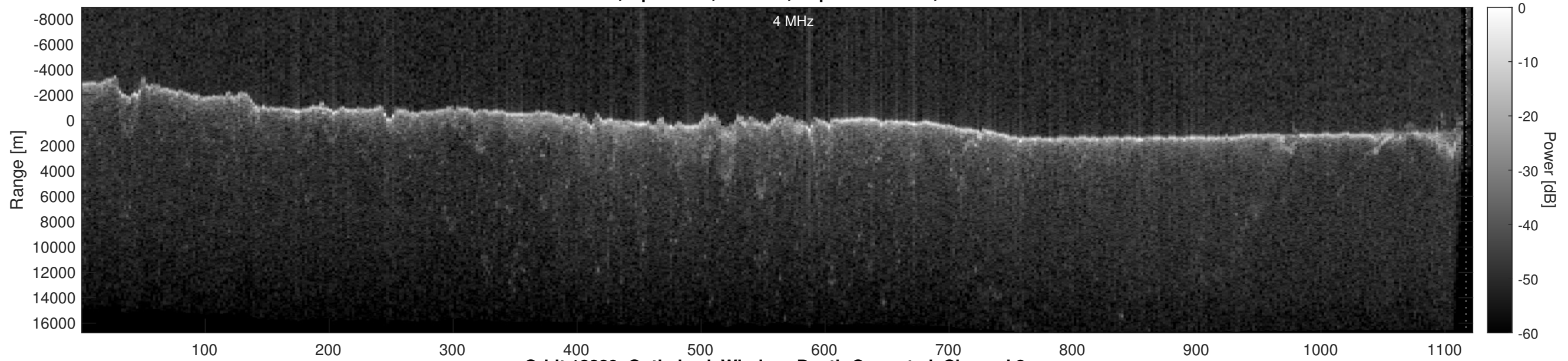
Orbit 12229, Optimized, Window, Depth-Corrected, Channel 2
