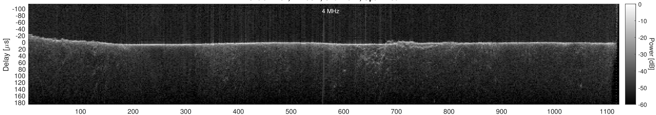
Orbit 12231, Cluttergram
