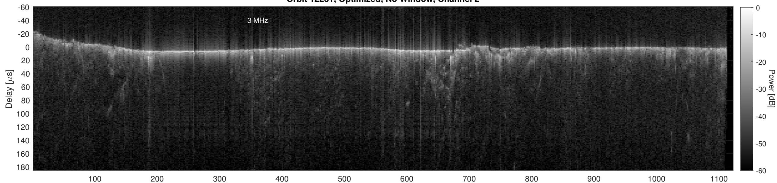
Orbit 12231, Cluttergram
