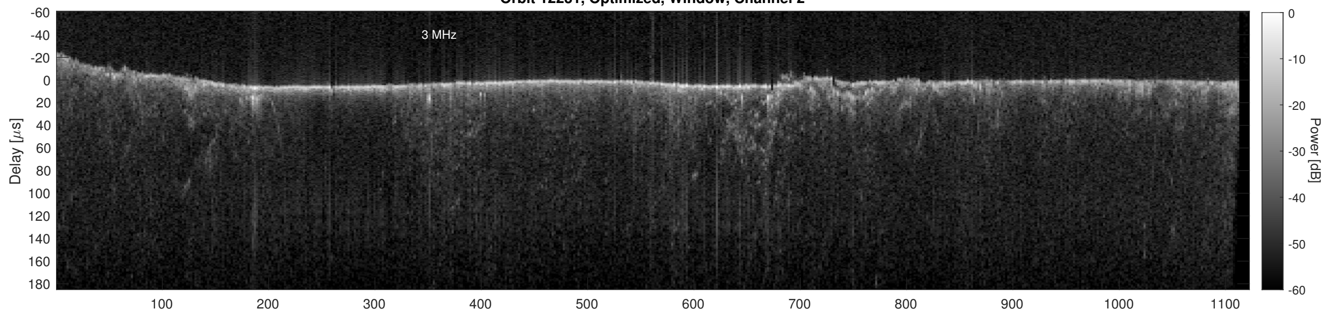
Orbit 12231, Cluttergram
