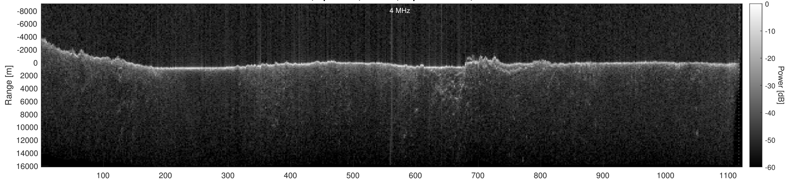
Orbit 12231, Optimized, Window, Depth-Corrected, Channel 2
