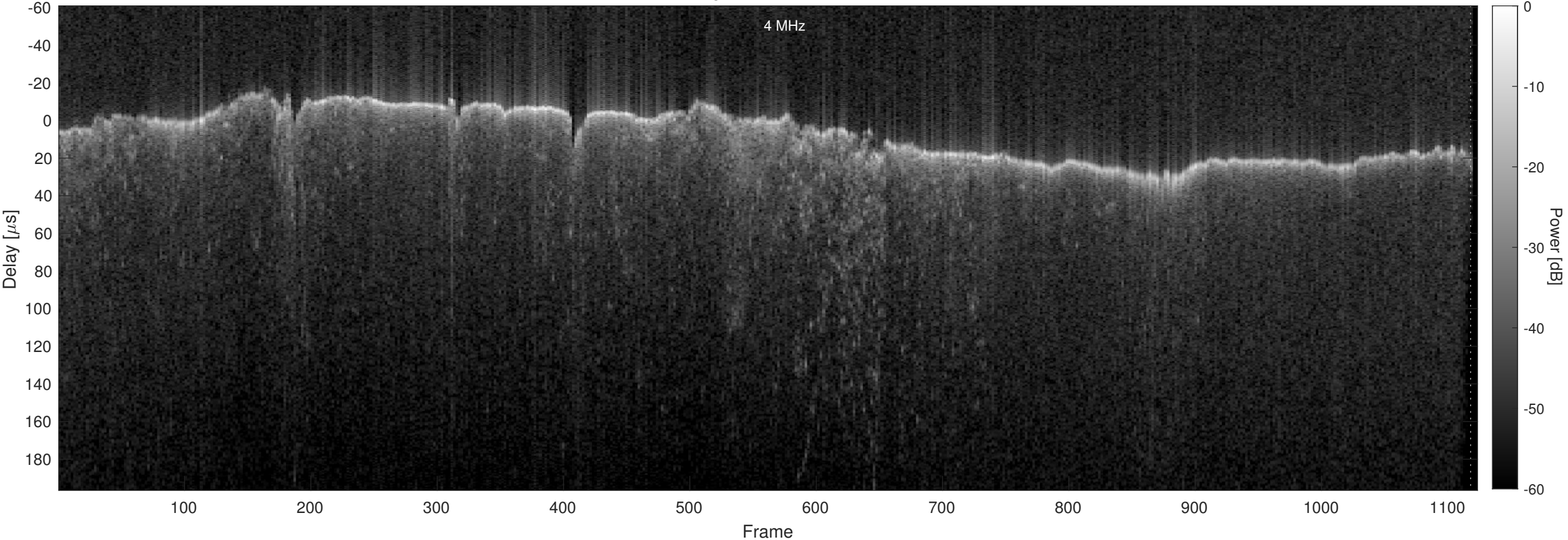
Orbit 12232, Chapman, No Window, Channel 2
