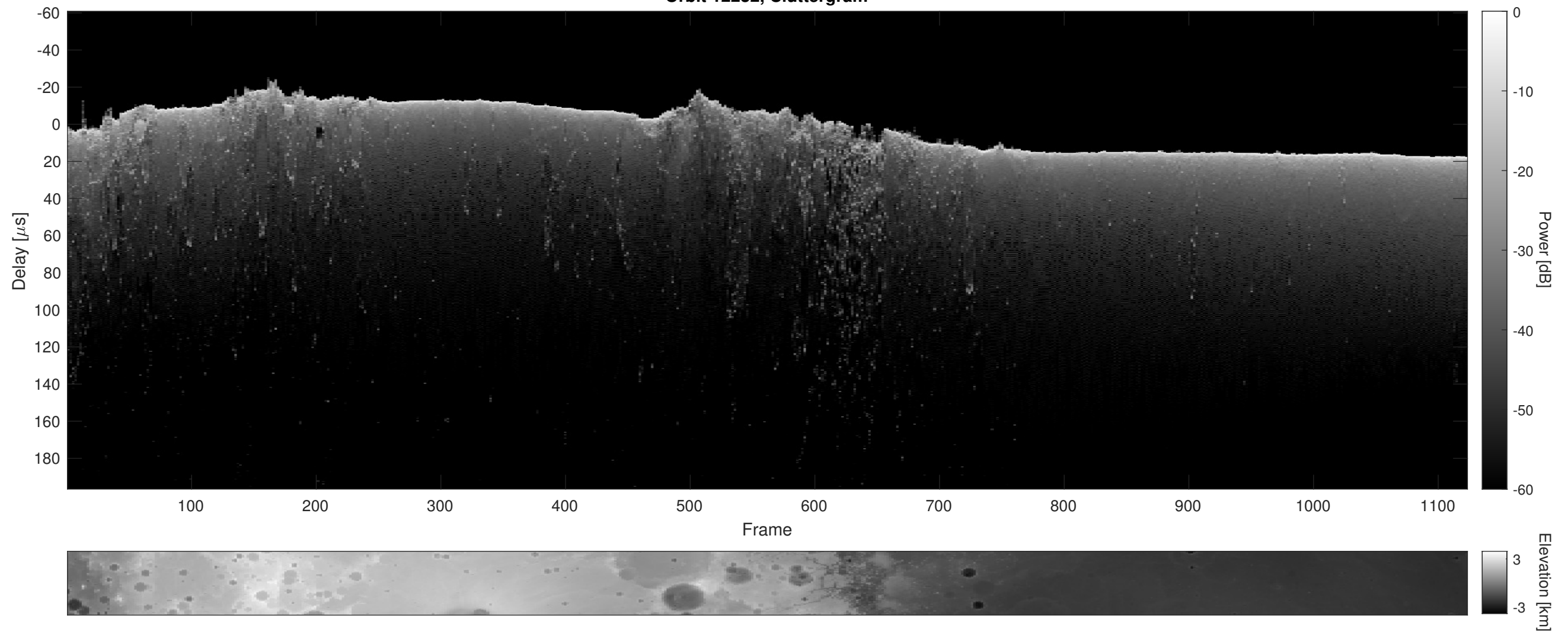
Orbit 12232, Cluttergram
