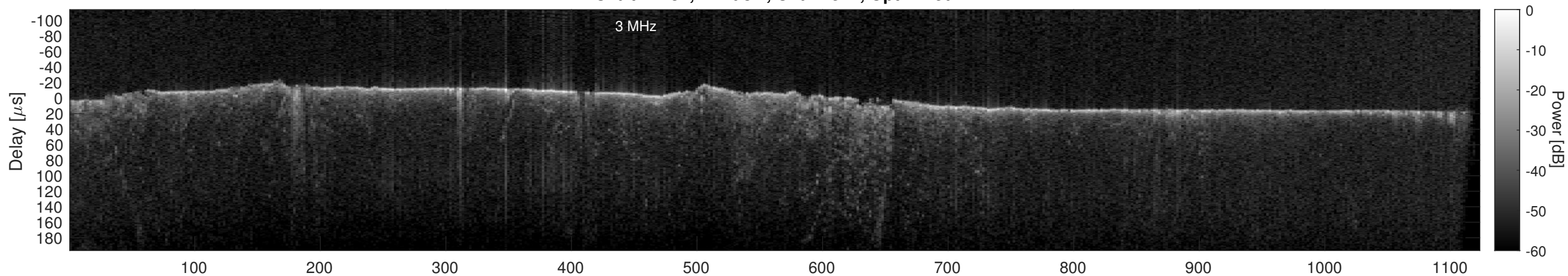
Orbit 12232, Cluttergram
