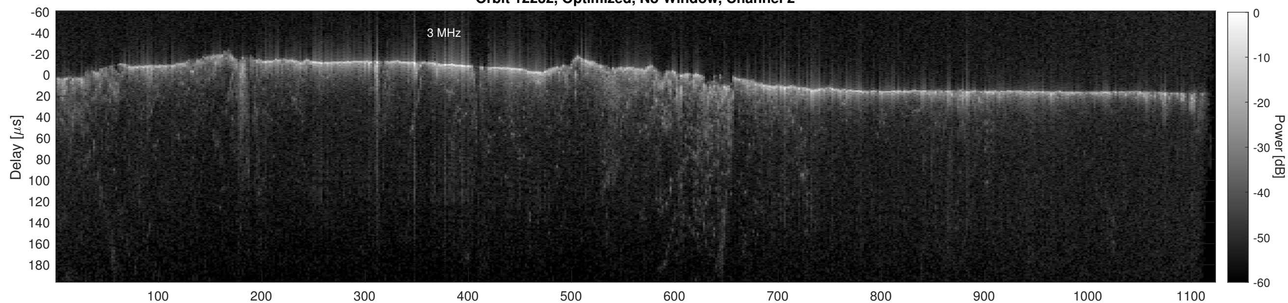
Orbit 12232, Cluttergram
