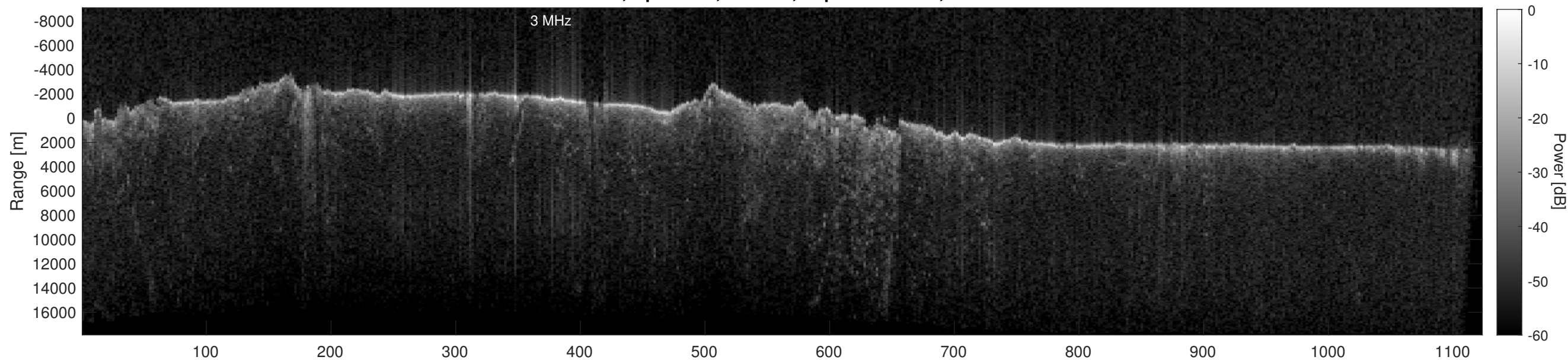
Orbit 12232, Depth-Corrected Cluttergram
