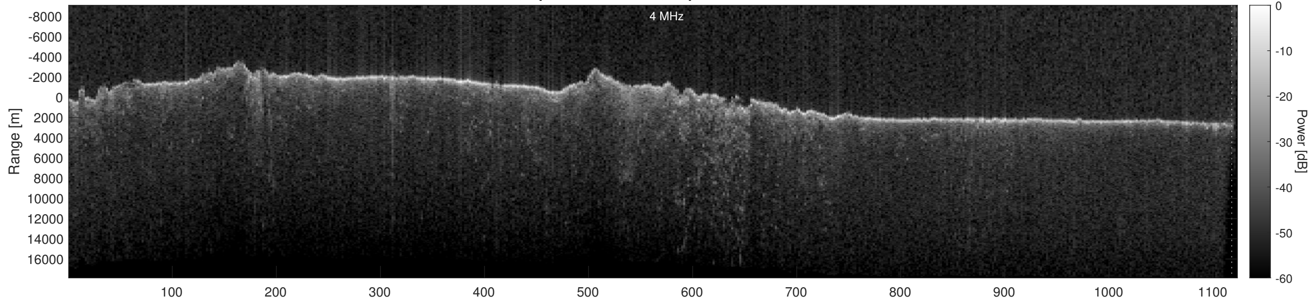
Orbit 12232, Optimized, Window, Depth-Corrected, Channel 2
