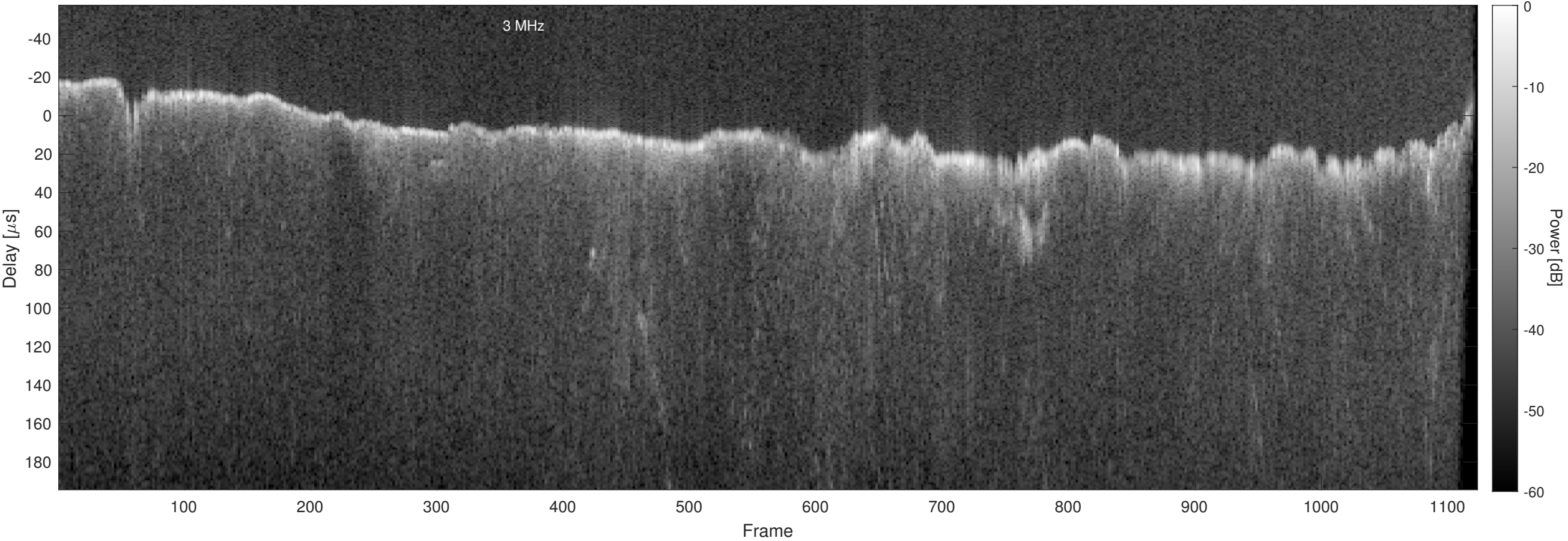
Orbit 12234, Chapman, Window, Channel 2
