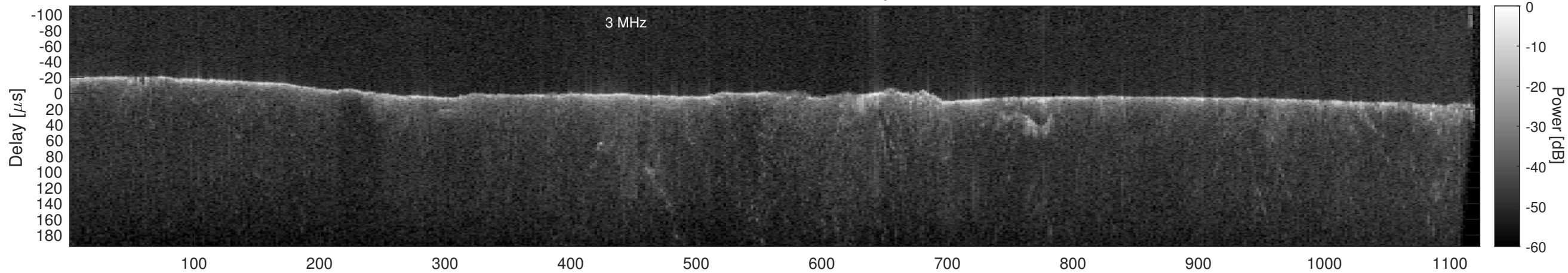
Orbit 12234, Cluttergram
