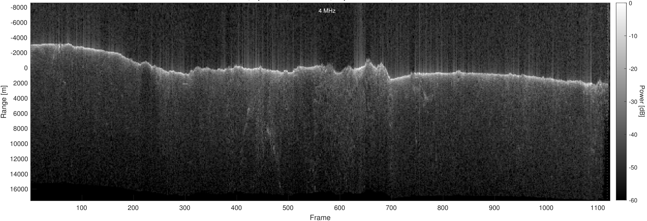
Orbit 12234, Optimized, No Window, Depth-Corrected, Channel 2
