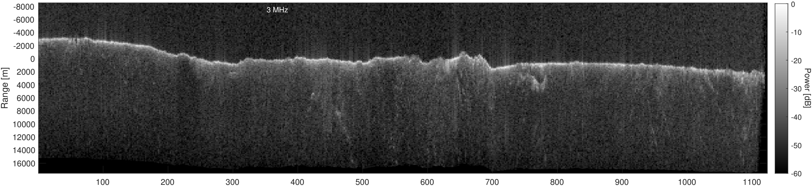
Orbit 12234, Depth-Corrected Cluttergram
