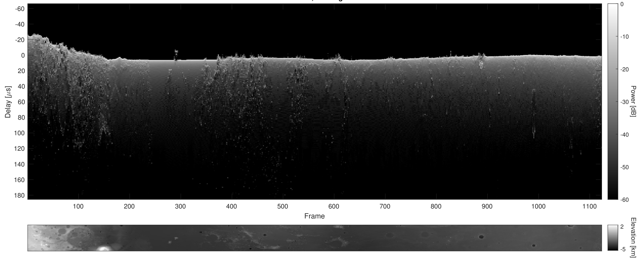
Orbit 12238, Cluttergram
