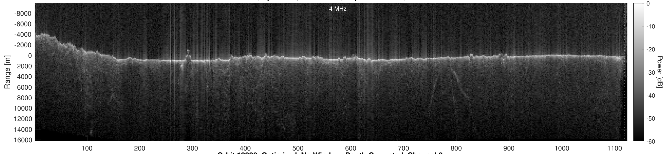
Orbit 12238, Optimized, No Window, Depth-Corrected, Channel 2
