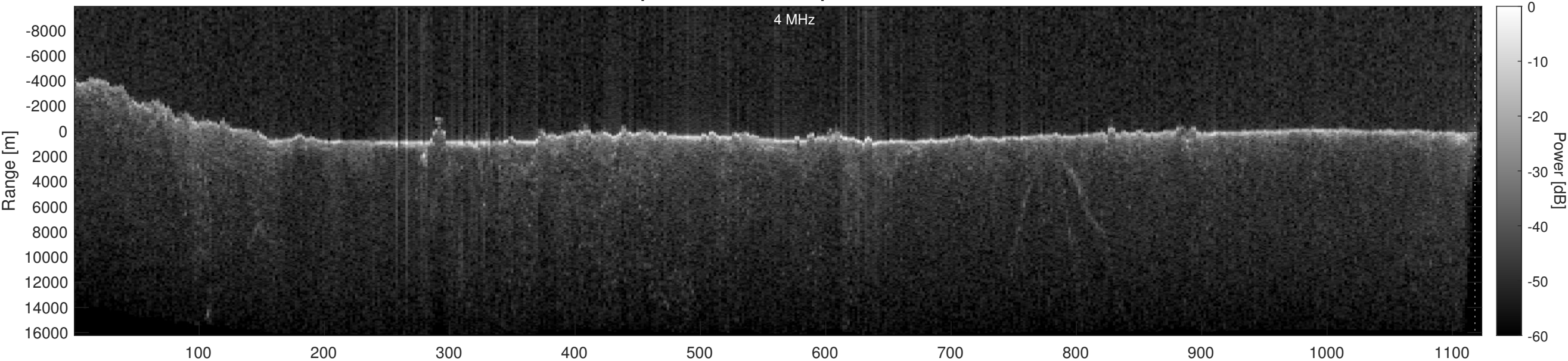
Orbit 12238, Optimized, Window, Depth-Corrected, Channel 2
