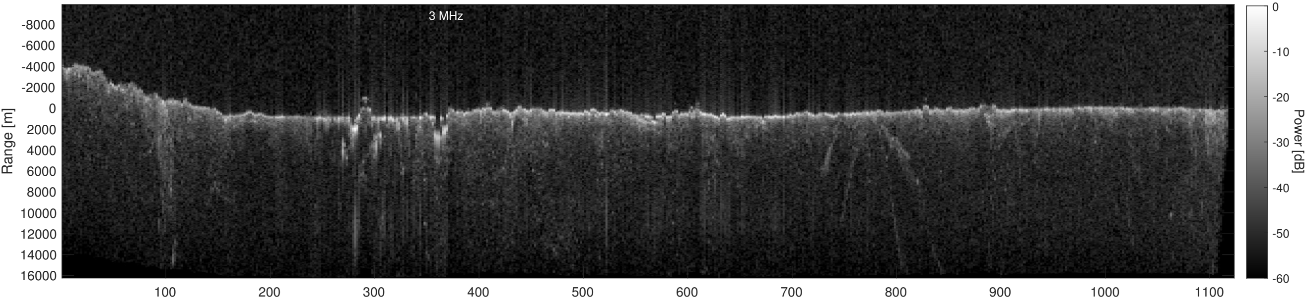
Orbit 12238, Depth-Corrected Cluttergram
