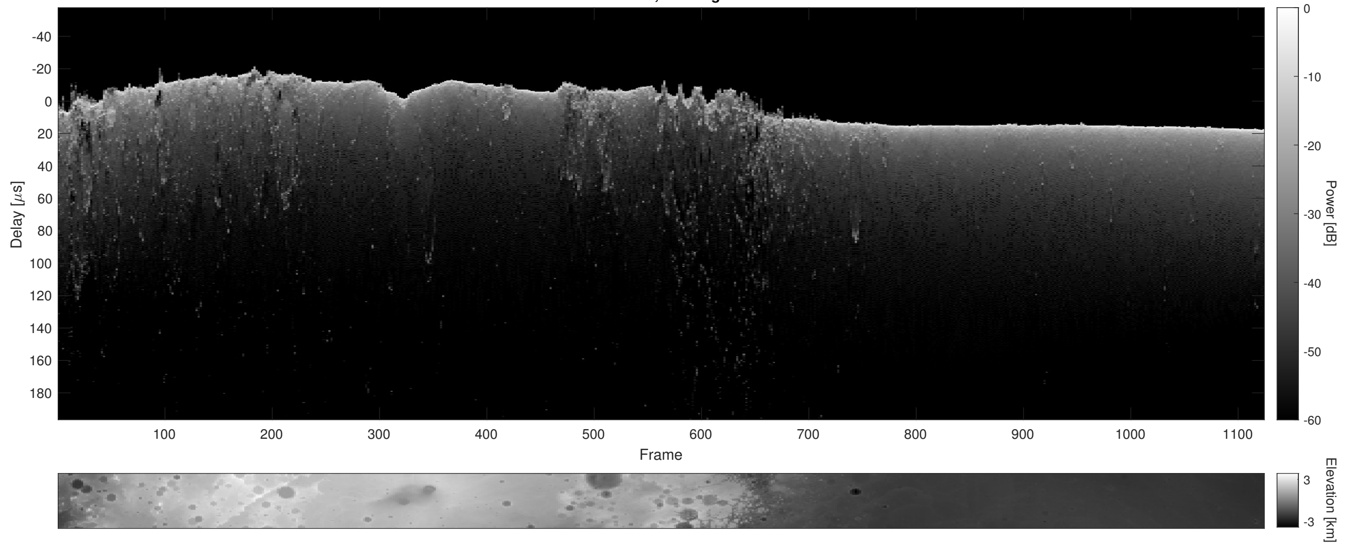
Orbit 12239, Cluttergram
