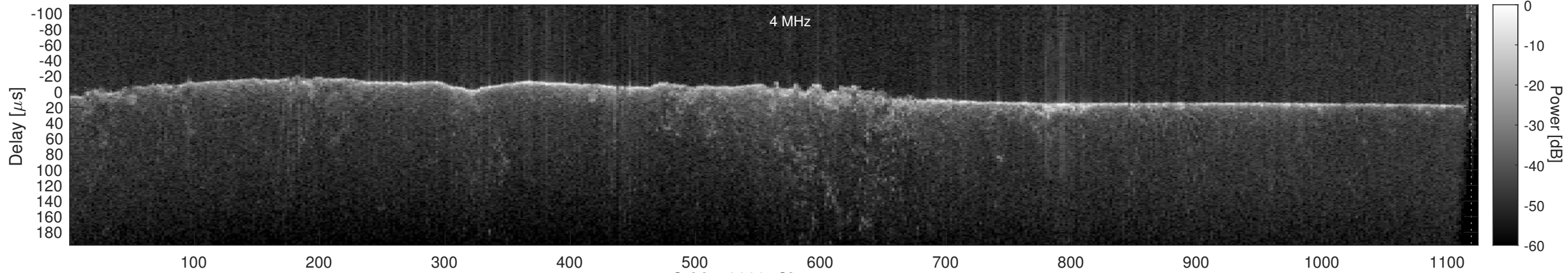
Orbit 12239, Cluttergram
