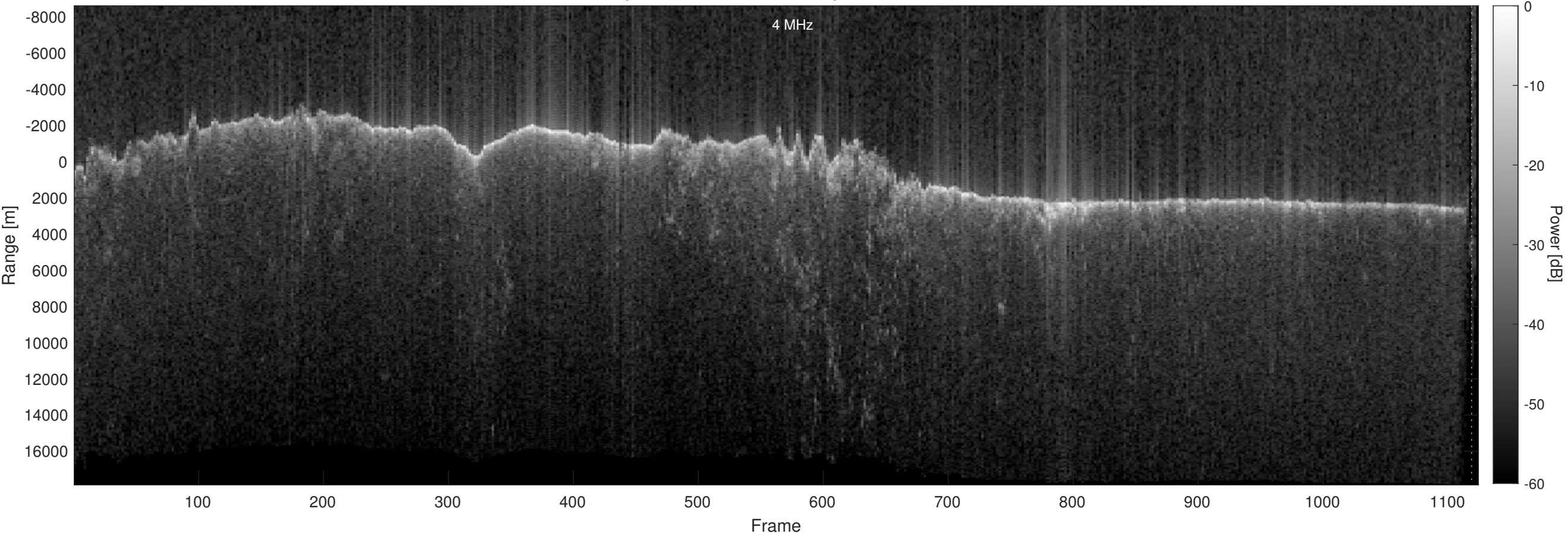
Orbit 12239, Optimized, No Window, Depth-Corrected, Channel 2
