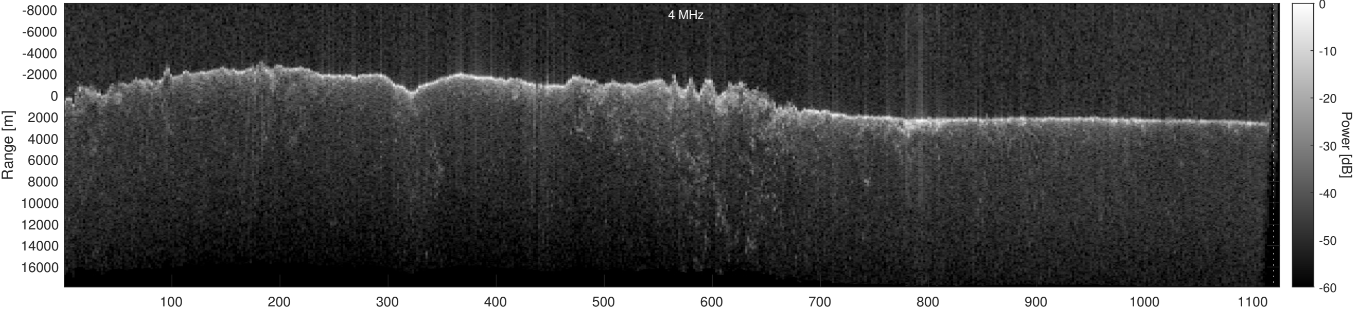
Orbit 12239, Optimized, Window, Depth-Corrected, Channel 2
