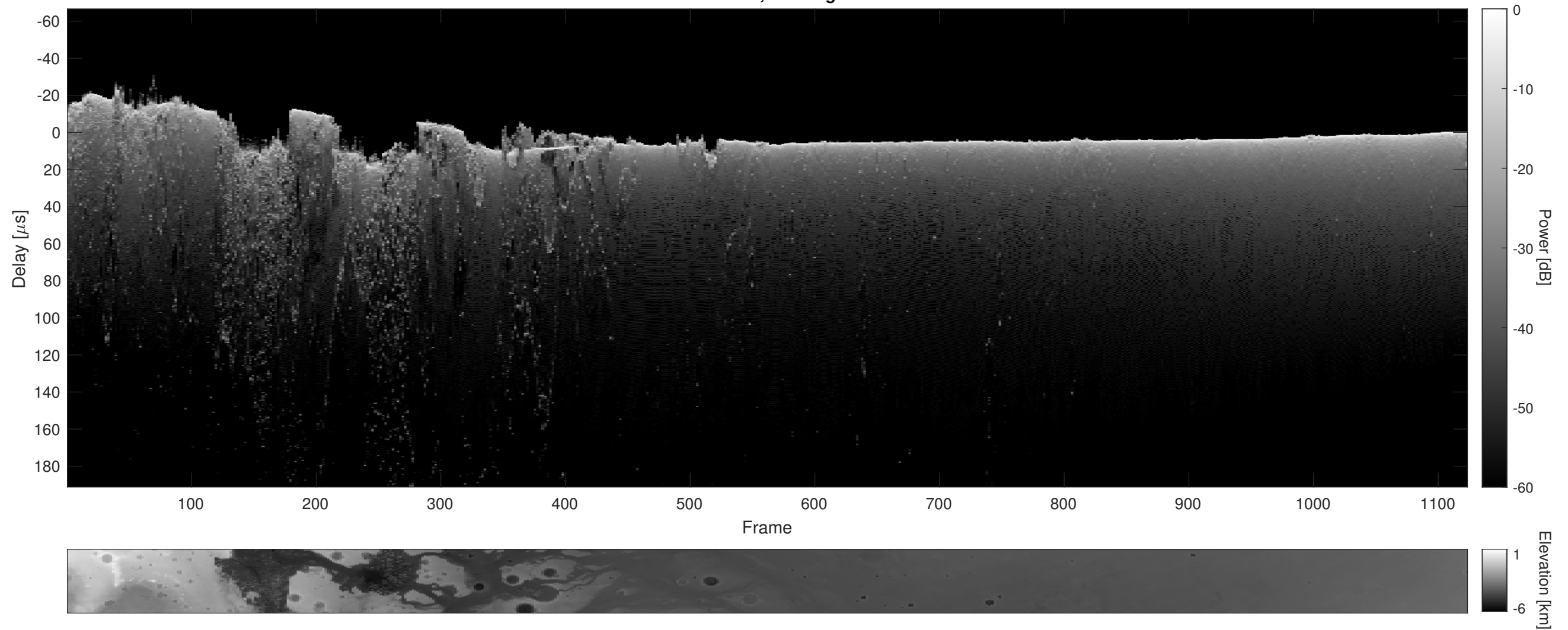
Orbit 12240, Cluttergram
