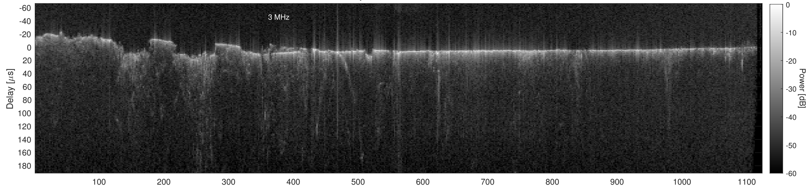
Orbit 12240, Cluttergram
