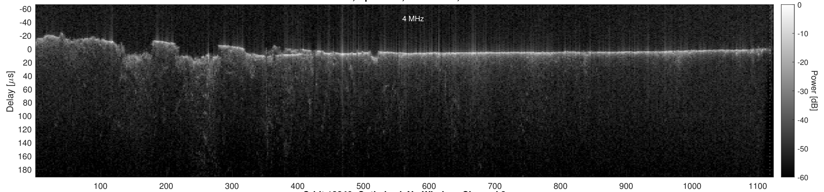
Orbit 12240, Optimized, No Window, Channel 2
